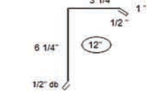
GABLE END COVERS - 12"
