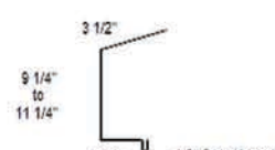
FASCIA FLASHING - 16"
