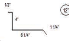
APRON WALL FLASHING - 12"
