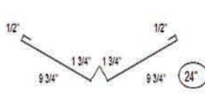
VALLEY GUTTER FLASHING - 24"
