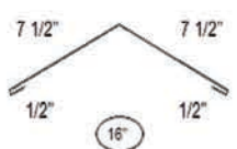
RIDGE CAP/HIP CAP - 16"
